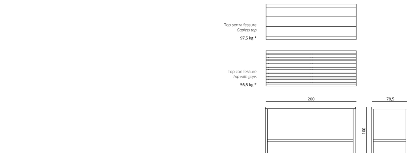
Tavolo free-standing alto / High free-standing table
